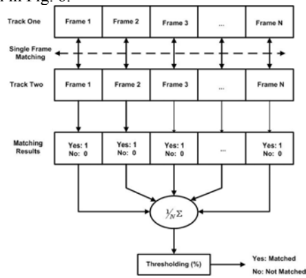
Figure 6 Single-frame matching and post-matching integration algorithms.
