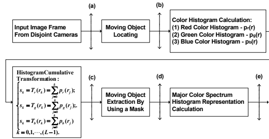
Figure 2 Moving objects image pre-processing for disjoint cameras
