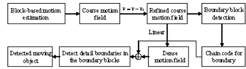
Fig. 1. process of moving object detection algorithm
