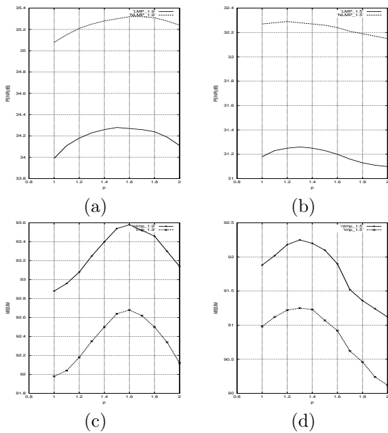
Figure 1: a) PSNR versus p for Lenna corrupted with S\alpha S \alpha = 1.9 . b) PSNR versus Lenna corrupted with S\alpha S \alpha = 1.5 . c) MSSIM versus p for Lenna corrupted with S\alpha S \alpha = 1.9 . d) MSSIM versus Lenna corrupted with S\alpha S \alpha = 1.5
